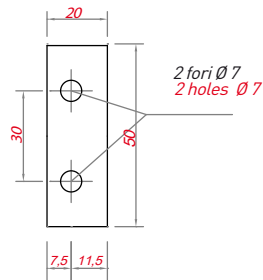
Staffa ancoraggio pannelli Panels assembling plate
